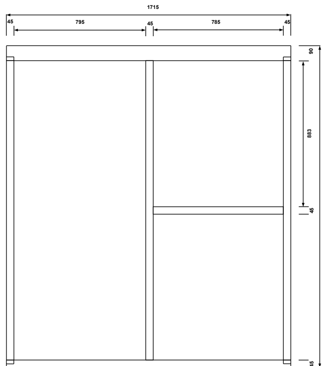
FRONT WALL
